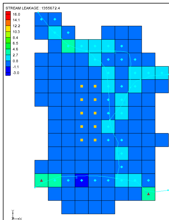
Figure 11 Block Fill showing stream in/out flow
