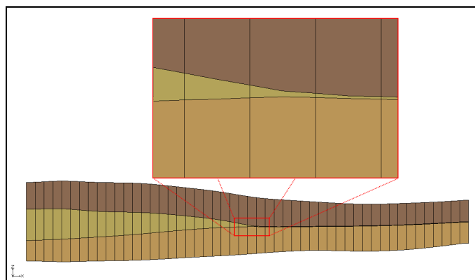
Figure 1 MODFLOW 2000 finite difference grid with pinching layer
