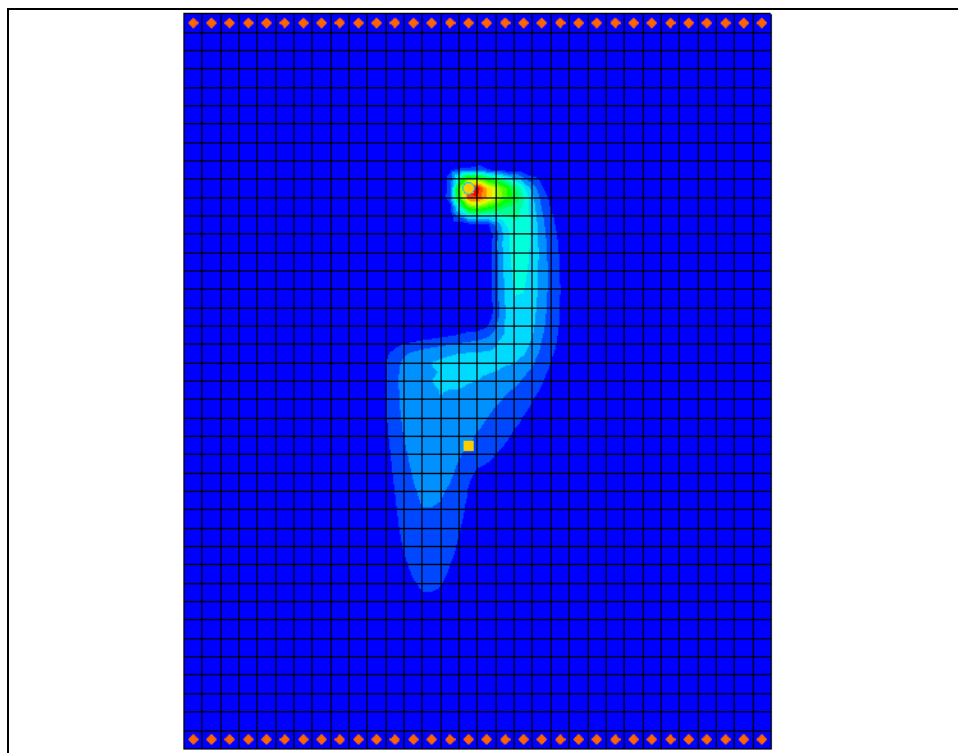
Figure 2 MT3D solution
