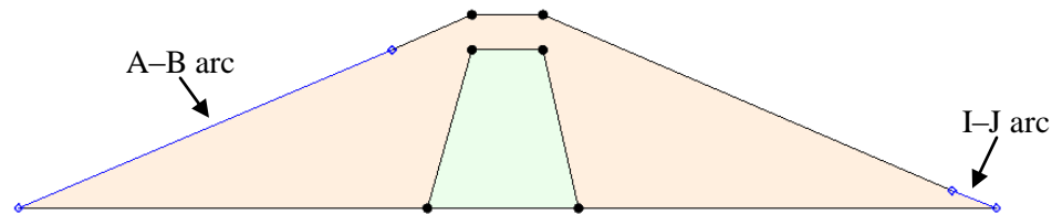
Figure 7 Specified-head boundaries
