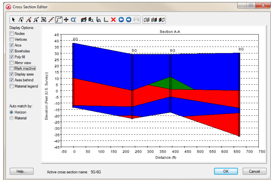
Figure 10 Multi-panel cross section ready for printing
