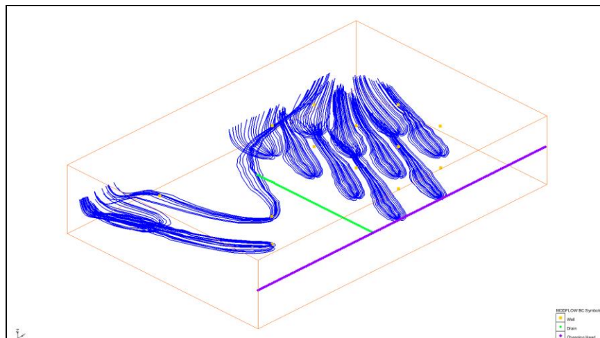
Figure 12 Pathline shapefile in 3D.
