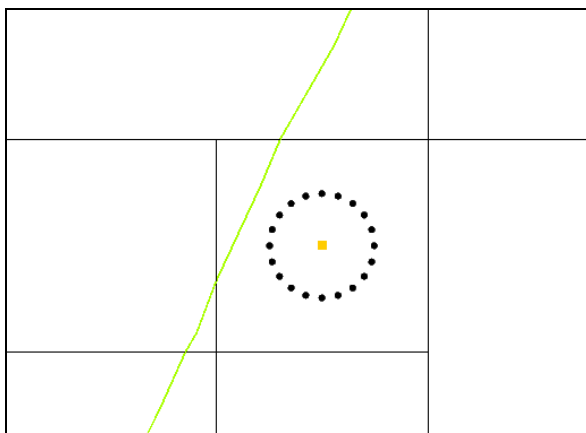
Figure 3 Ring of particle starting locations around wells
