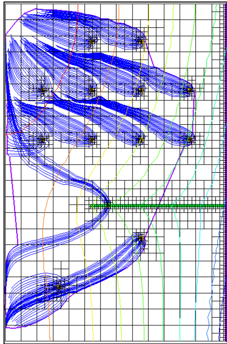
Figure 10 Pathline solution showing pathlines tracking backward from the well.
