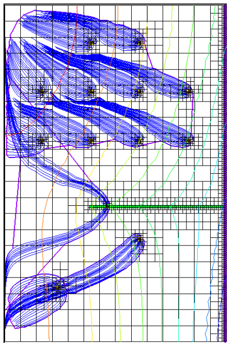
Figure 11 Capture zones for different well groups
